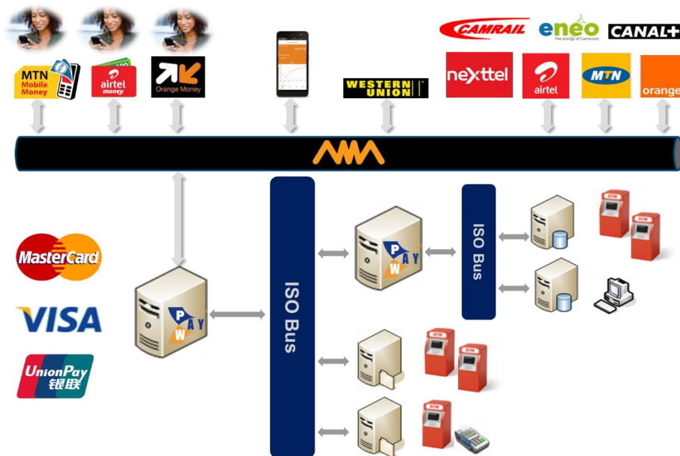
Figure 1: AMA platform architecture
